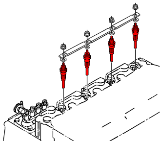
Glow plug
