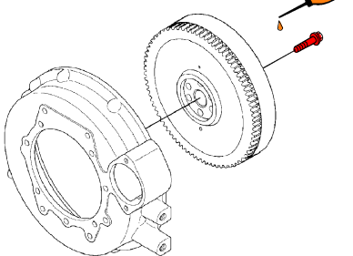
Flywheel screw *
